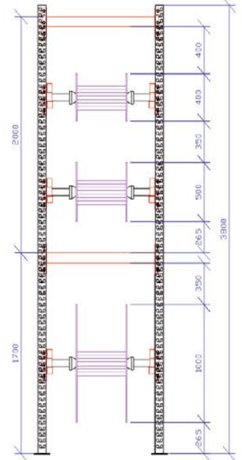
Height 3,800 mm
