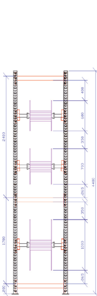
Height 4,400 mm
